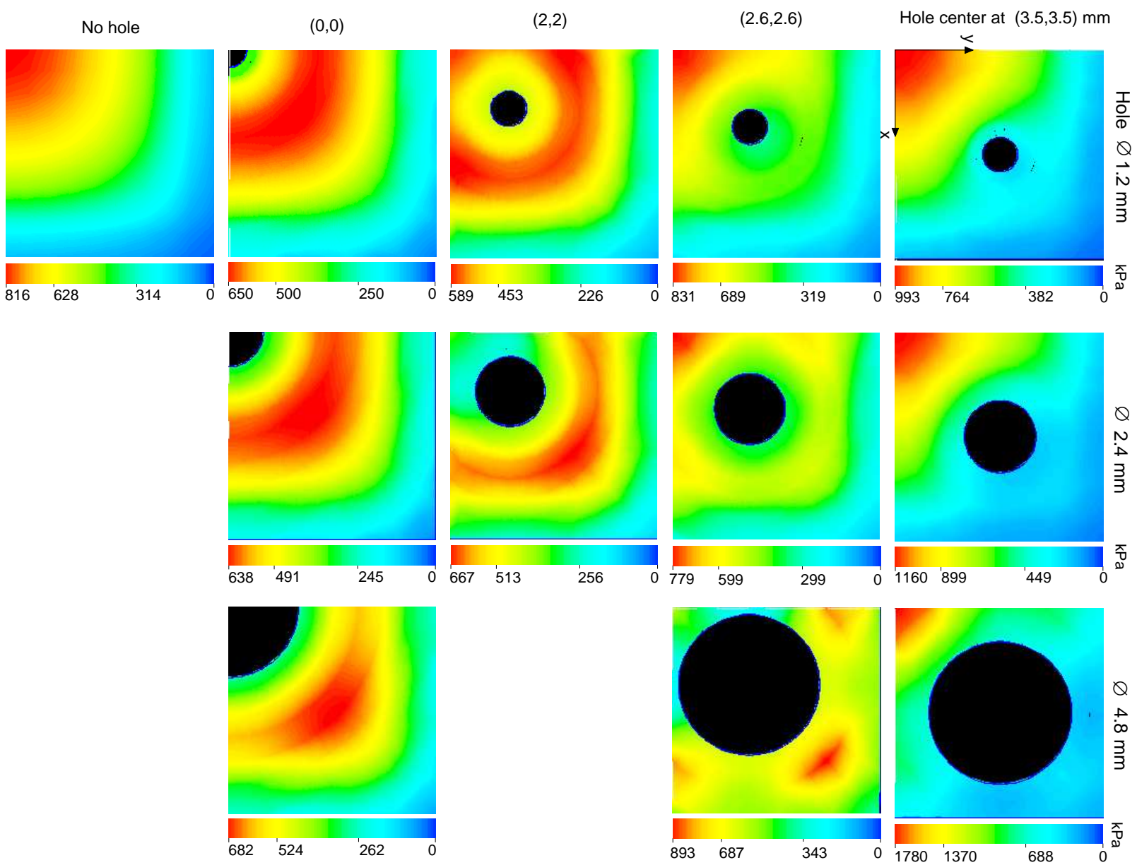
Figure 23: Normal contact stresses for various hole diameters and placement
