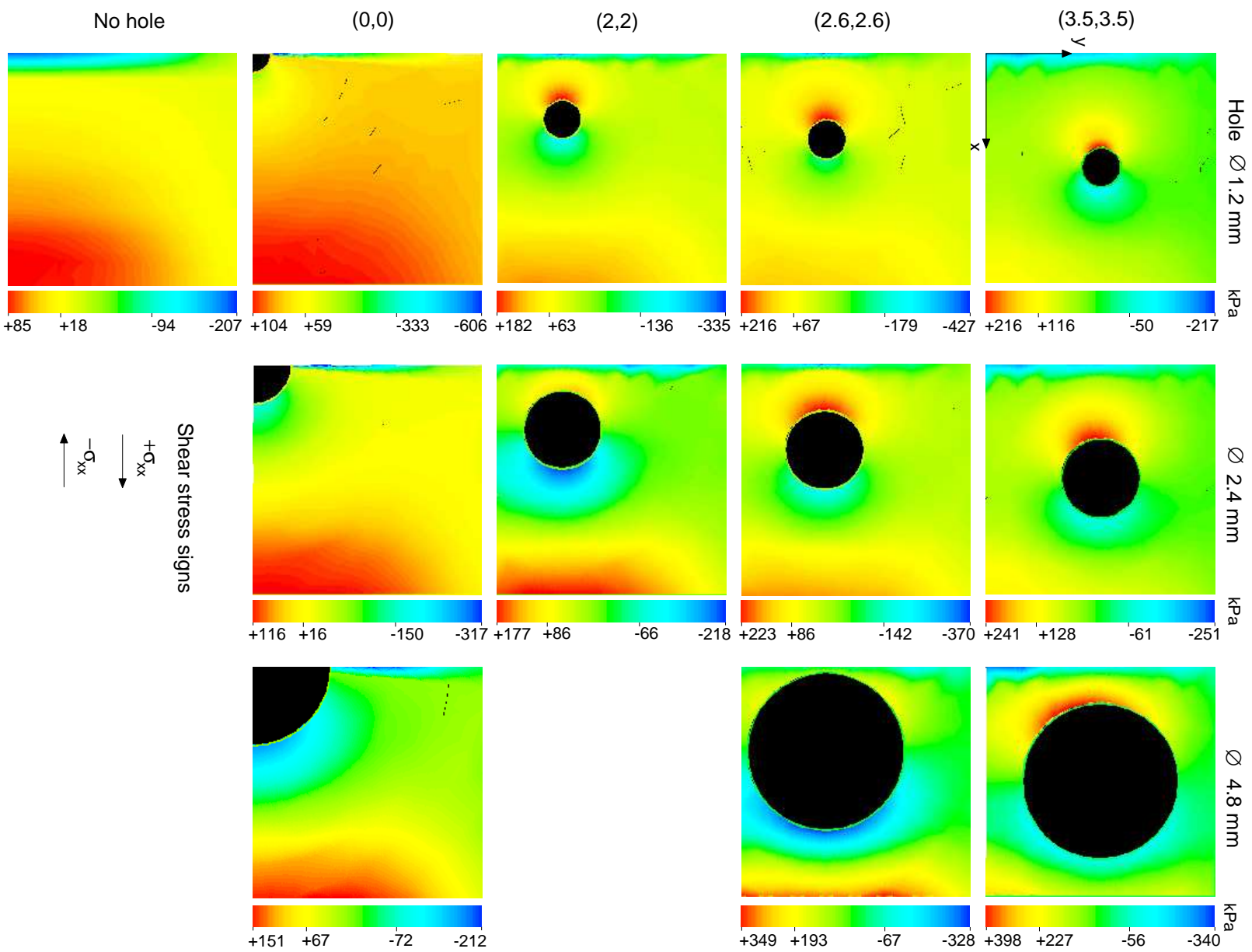
Figure 24: Shear contact stresses for various hole diameters and placement
