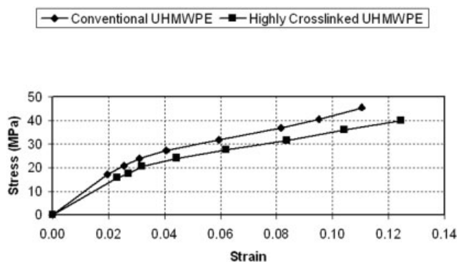
Figure 3. True stress/true strain conventional and highly crosslinked UHMWPE.
