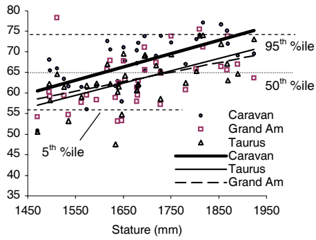
Figure 8. Bolster-to-femur angle at bolster contact to occupant stature for the Caravan, Grand Am and Taurus. Percentiles are from the combined data from all vehicles and occupants.
