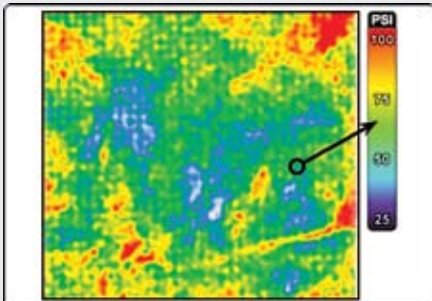
Pressurex® Pressure Profile after Image Analysis
