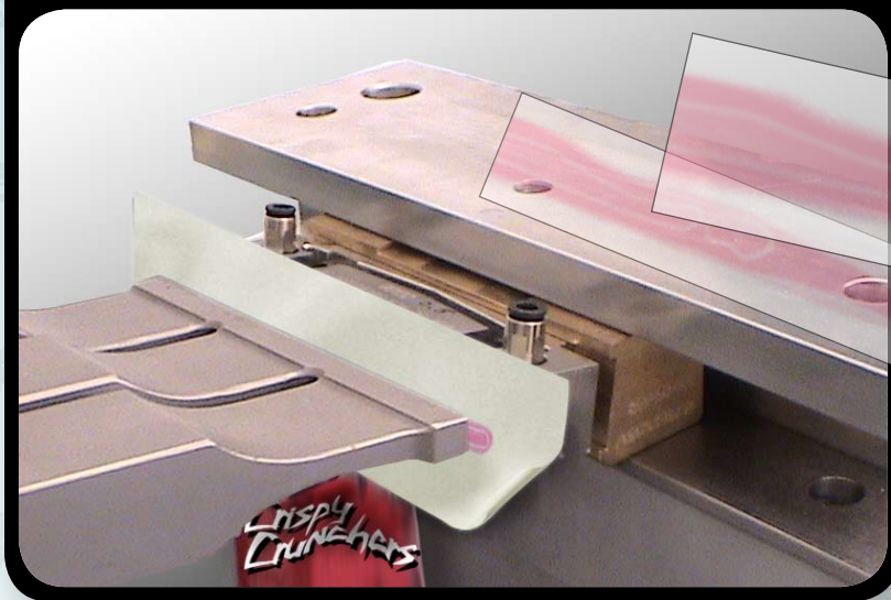
Pressure film in place in heat sealing device.
