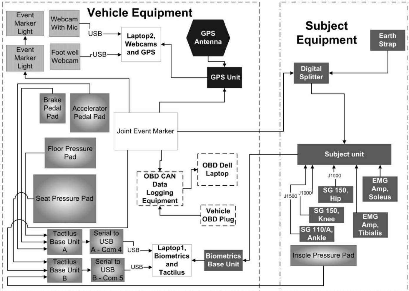
Figure 1. Ergonomic data measuring system architecture
